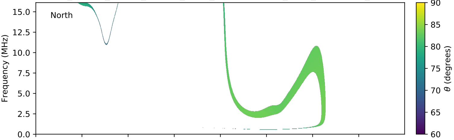
expres_cassini_jupiter_europa_isaac_lossc-wid1deg_3kev_20020205_v01.cdf
