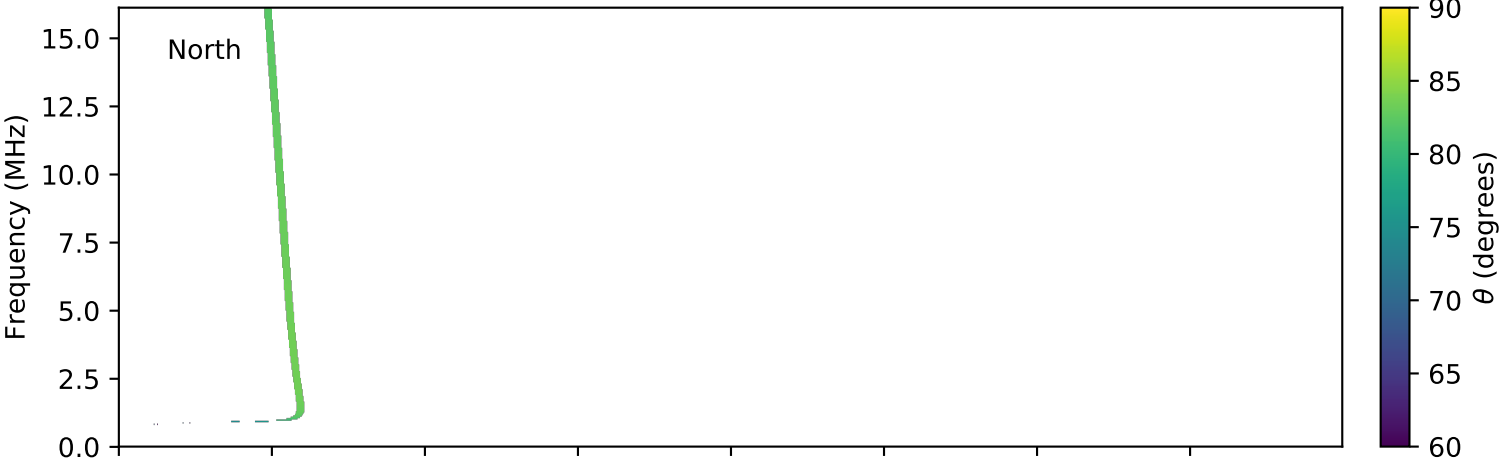
expres_cassini_jupiter_europa_isaac_lossc-wid1deg_3kev_20020202_v01.cdf
