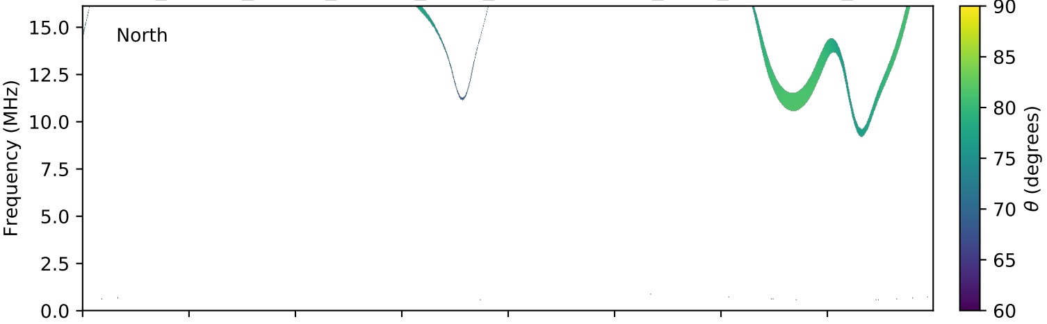
expres_cassini_jupiter_europa_isaac_lossc-wid1deg_3kev_20020201_v01.cdf
