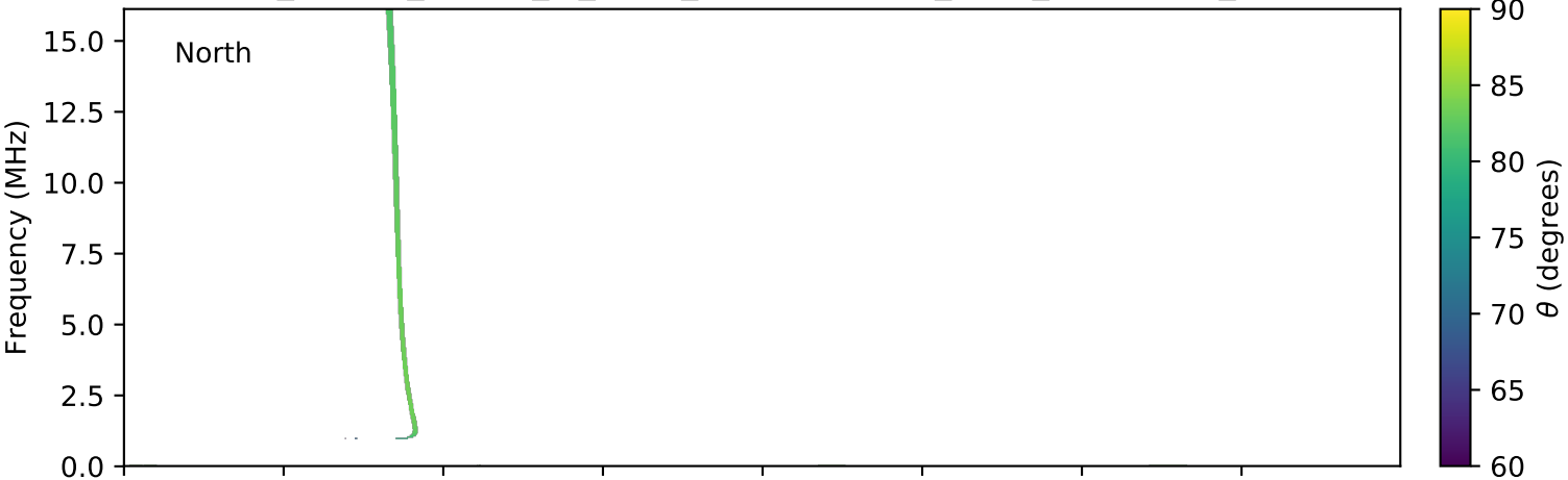
expres_cassini_jupiter_io_isaac_lossc-wid1deg_3kev_20020128_v01.cdf
