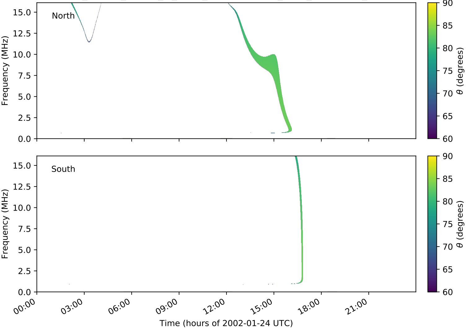
expres_cassini_jupiter_io_isaac_lossc-wid1deg_3kev_20020124_v01.cdf
