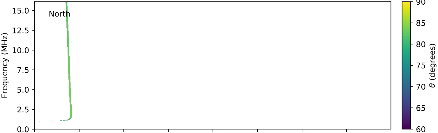
expres_cassini_jupiter_io_isaac_lossc-wid1deg_3kev_20020114_v01.cdf
