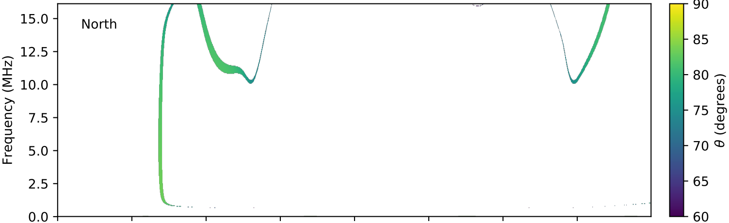
expres_cassini_jupiter_io_isaac_lossc-wid1deg_3kev_20020106_v01.cdf
