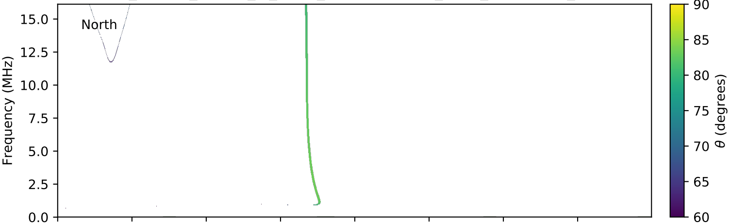
expres_cassini_jupiter_io_isaac_lossc-wid1deg_3kev_20020103_v01.cdf
