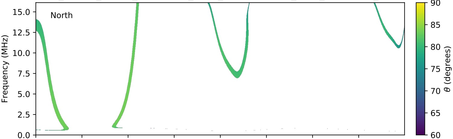
expres_cassini_jupiter_ganymede_isaac_lossc-wid1deg_3kev_20020131_v01.cdf
