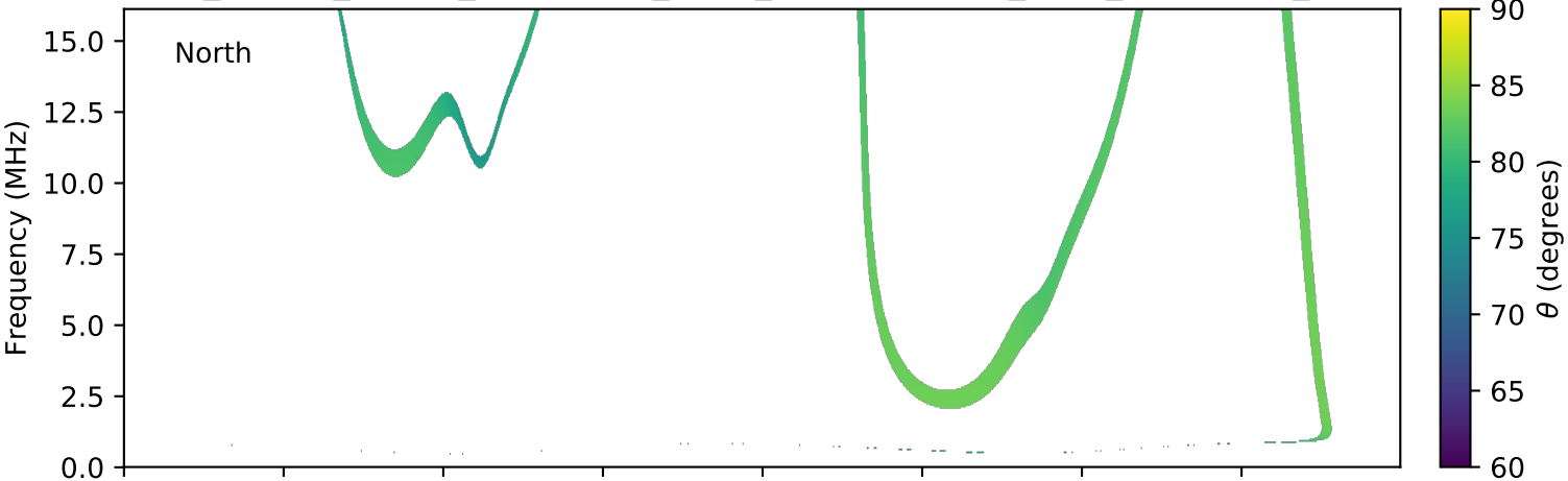
expres_cassini_jupiter_ganymede_isaac_lossc-wid1deg_3kev_20020126_v01.cdf
