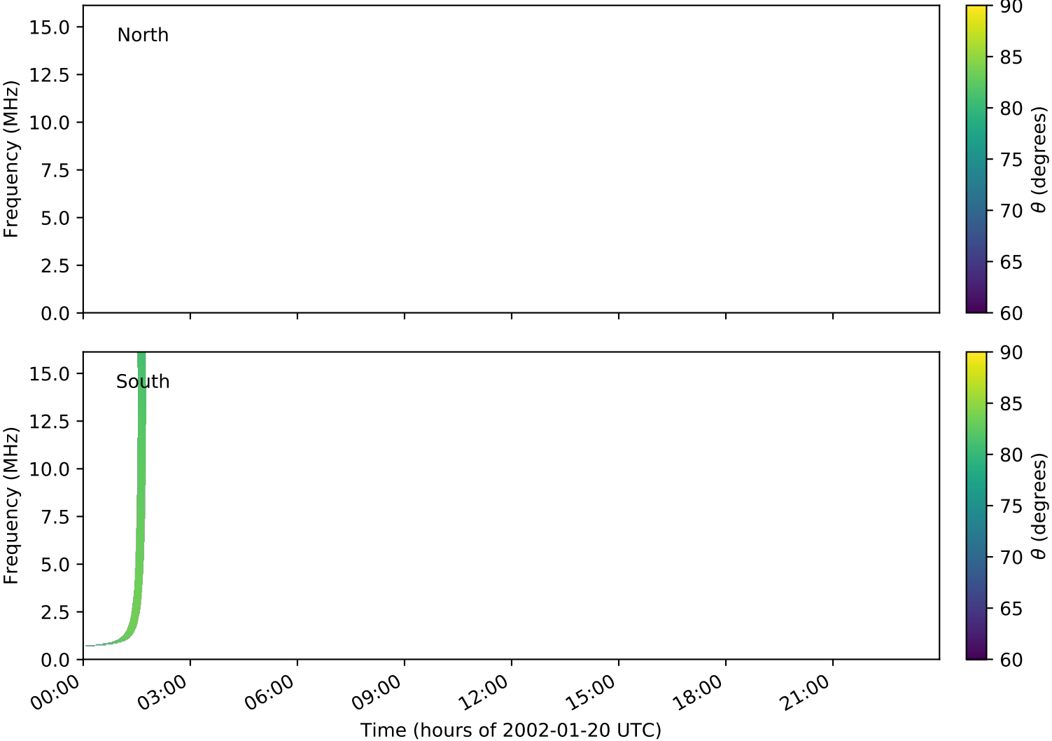
expres_cassini_jupiter_ganymede_isaac_lossc-wid1deg_3kev_20020120_v01.cdf
