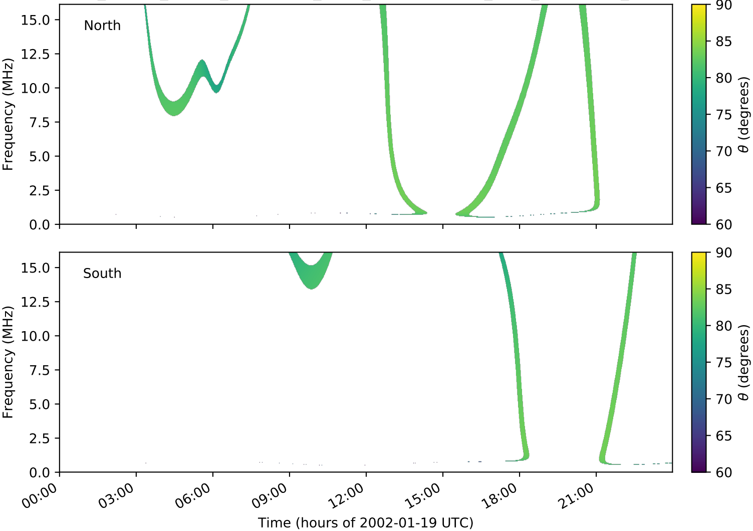
expres_cassini_jupiter_ganymede_isaac_lossc-wid1deg_3kev_20020119_v01.cdf
