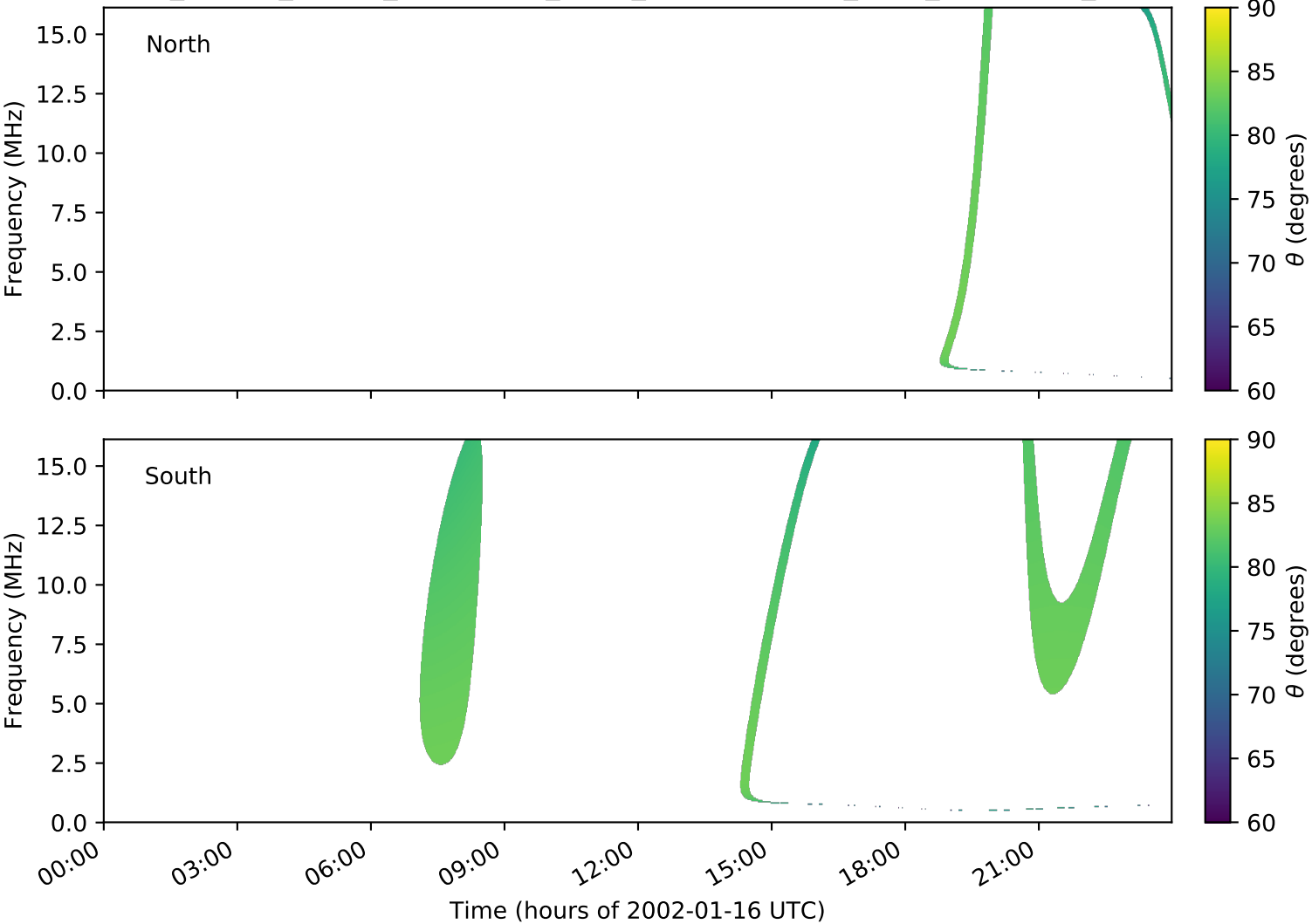
expres_cassini_jupiter_ganymede_isaac_lossc-wid1deg_3kev_20020116_v01.cdf
