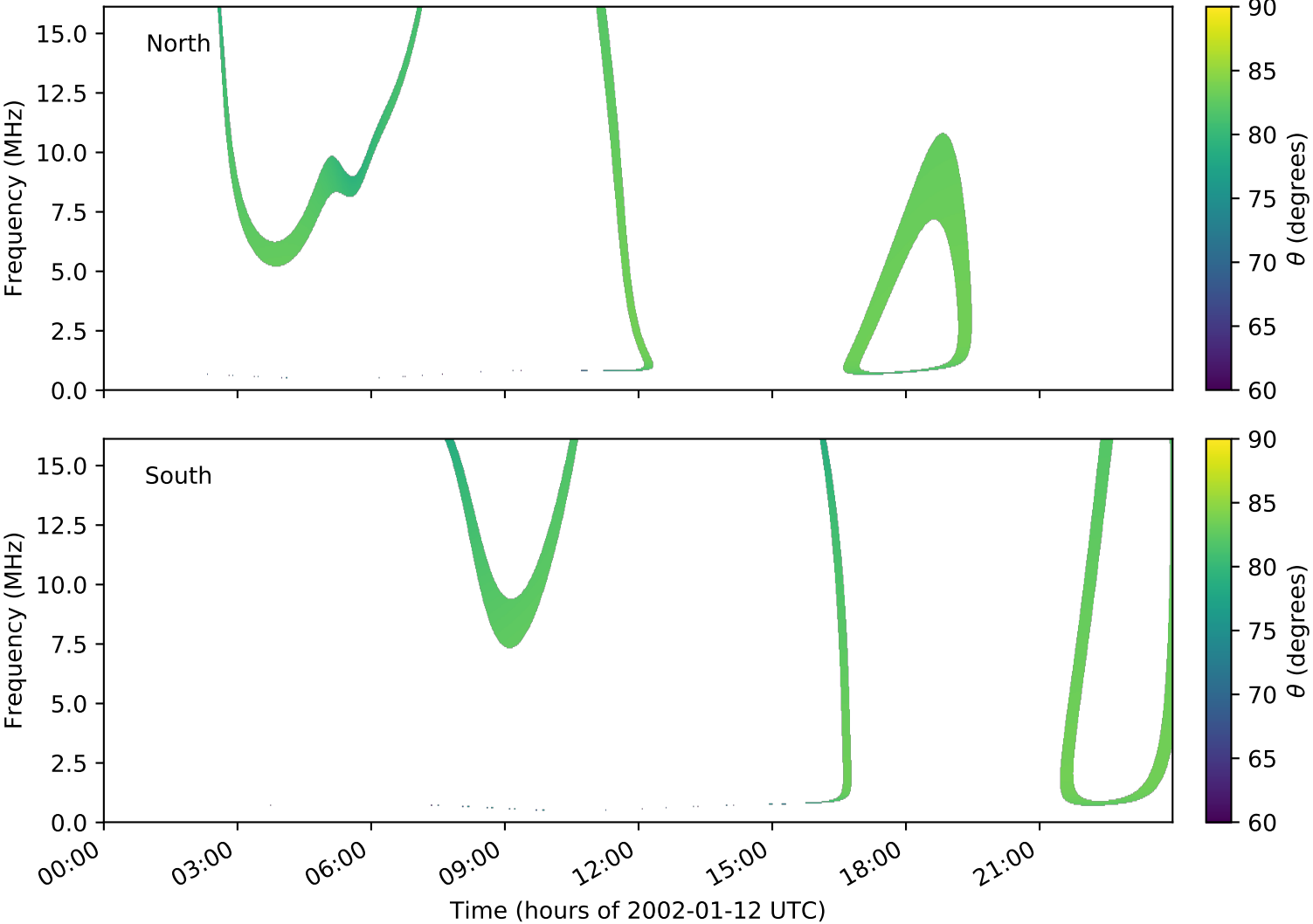
expres_cassini_jupiter_ganymede_isaac_lossc-wid1deg_3kev_20020112_v01.cdf
