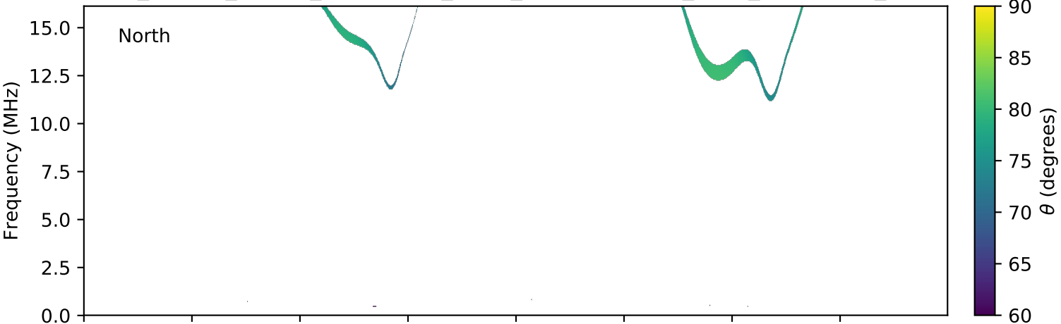
expres_cassini_jupiter_ganymede_isaac_lossc-wid1deg_3kev_20020111_v01.cdf
