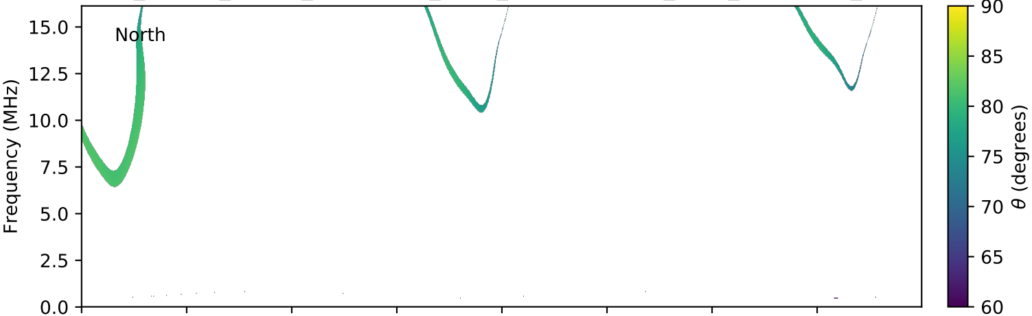
expres_cassini_jupiter_ganymede_isaac_lossc-wid1deg_3kev_20020110_v01.cdf
