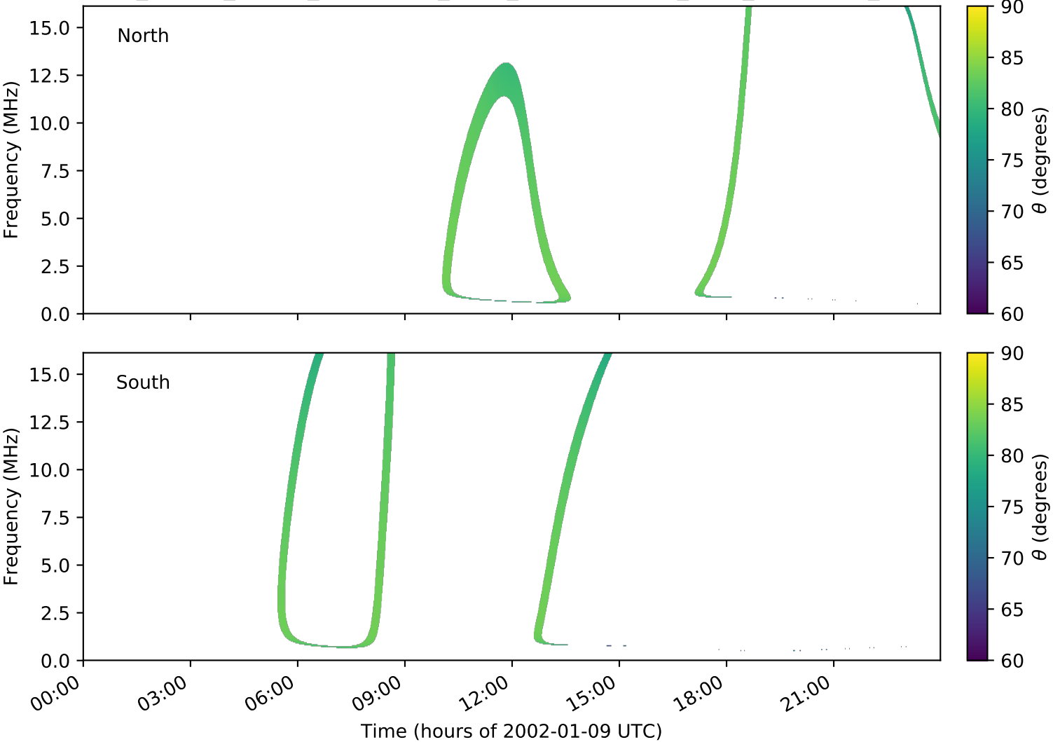
expres_cassini_jupiter_ganymede_isaac_lossc-wid1deg_3kev_20020109_v01.cdf
