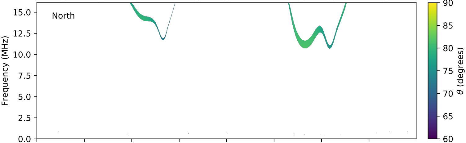
expres_cassini_jupiter_ganymede_isaac_lossc-wid1deg_3kev_20020104_v01.cdf
