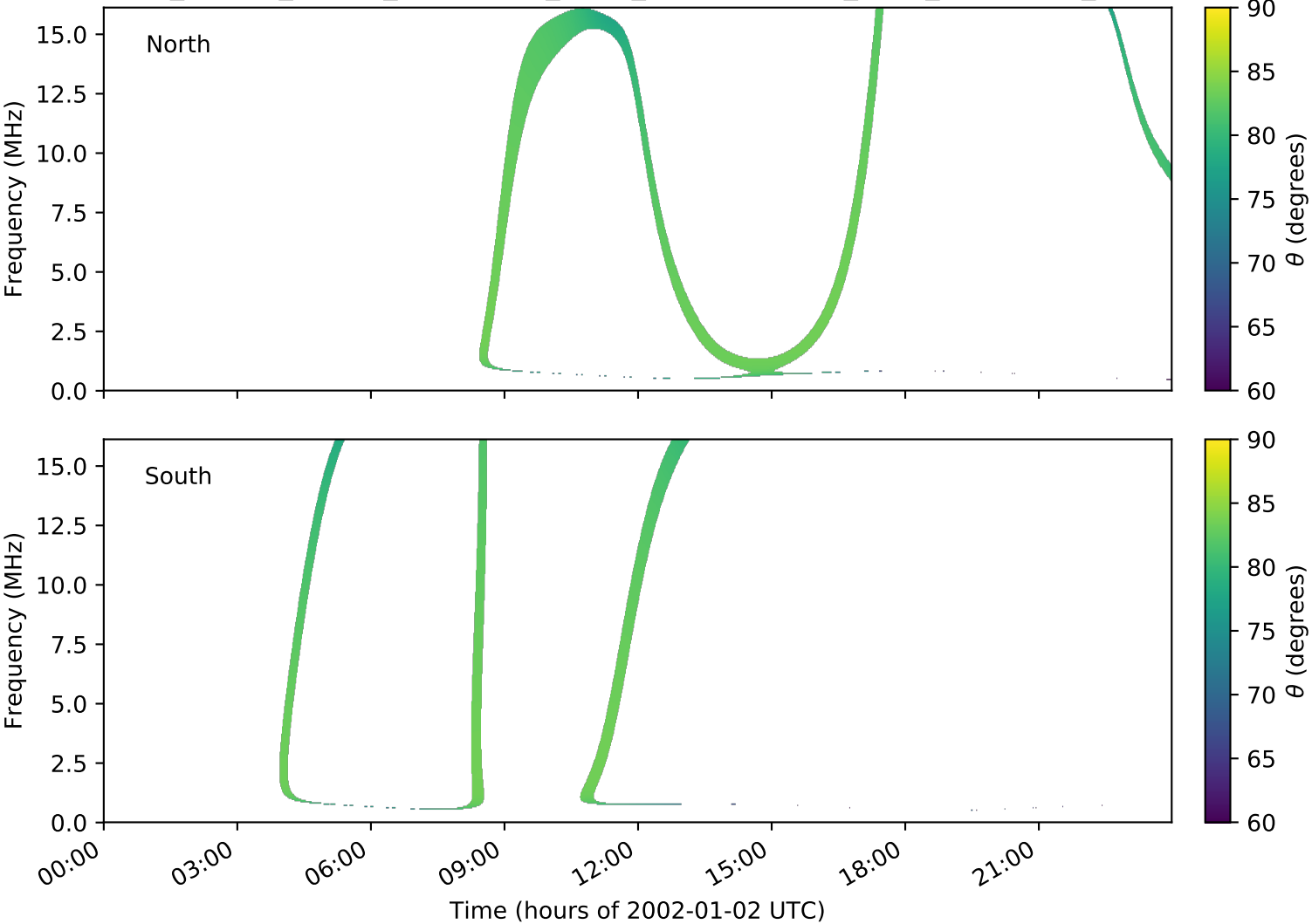
expres_cassini_jupiter_ganymede_isaac_lossc-wid1deg_3kev_20020102_v01.cdf
