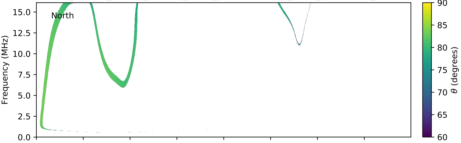
expres_cassini_jupiter_europa_isaac_lossc-wid1deg_3kev_20020128_v01.cdf
