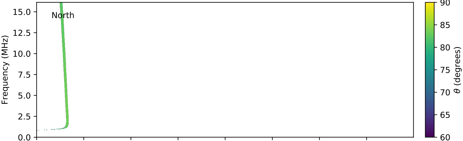
expres_cassini_jupiter_europa_isaac_lossc-wid1deg_3kev_20020126_v01.cdf
