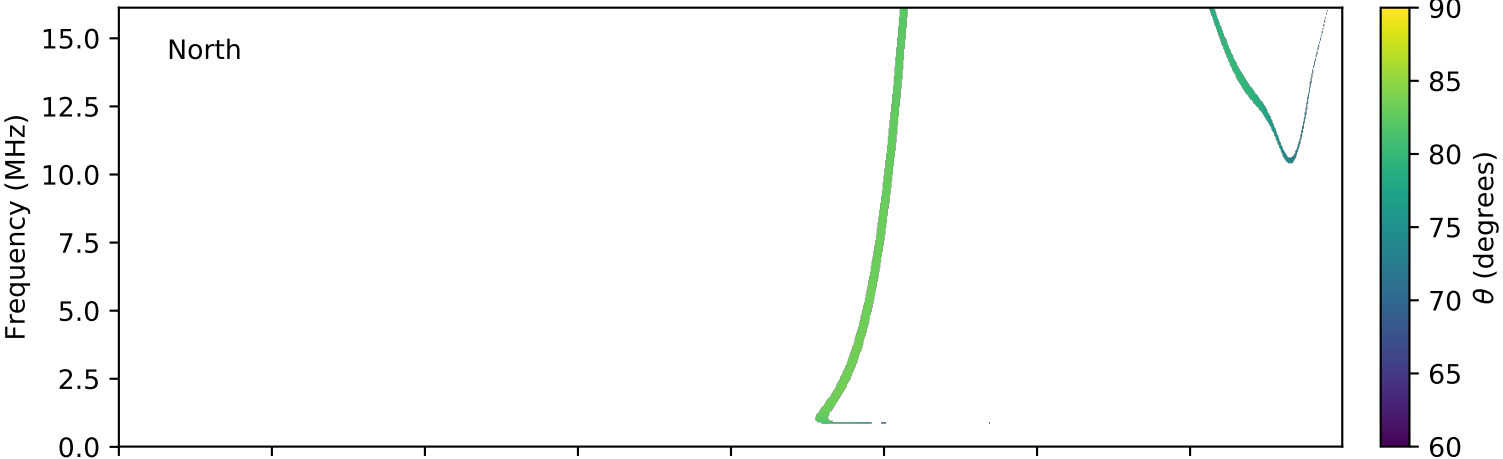
expres_cassini_jupiter_europa_isaac_lossc-wid1deg_3kev_20020124_v01.cdf
