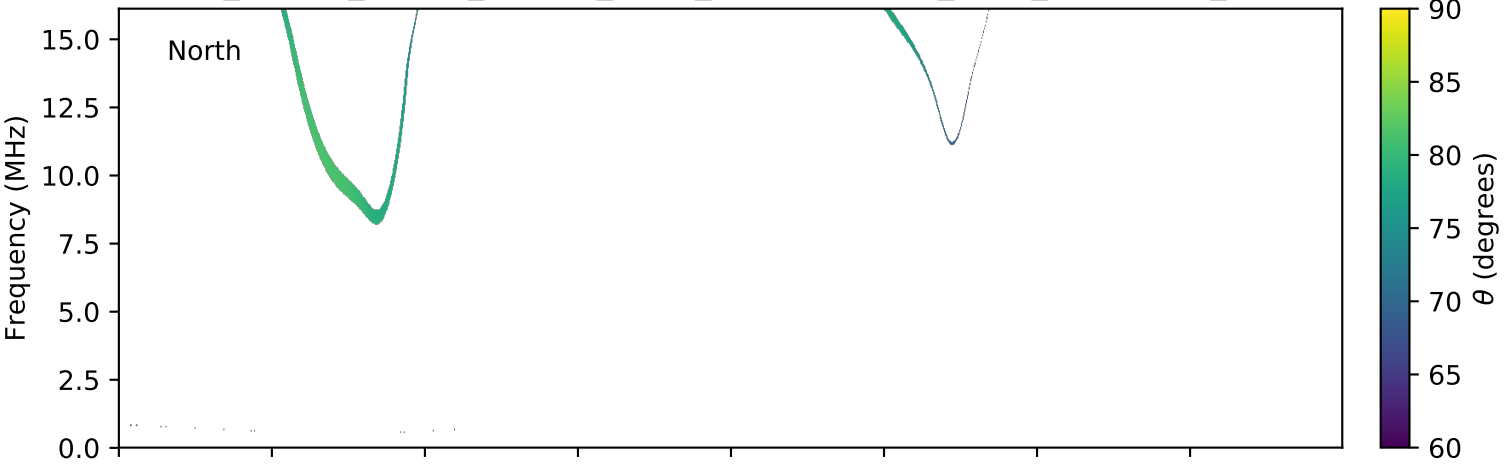
expres_cassini_jupiter_europa_isaac_lossc-wid1deg_3kev_20020121_v01.cdf
