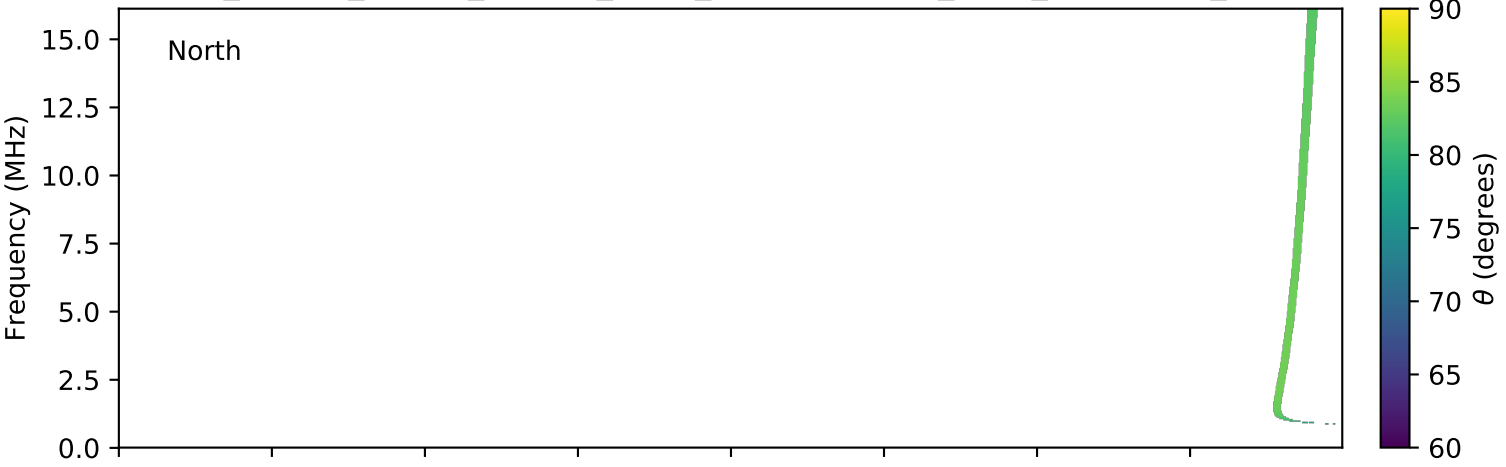
expres_cassini_jupiter_europa_isaac_lossc-wid1deg_3kev_20020120_v01.cdf
