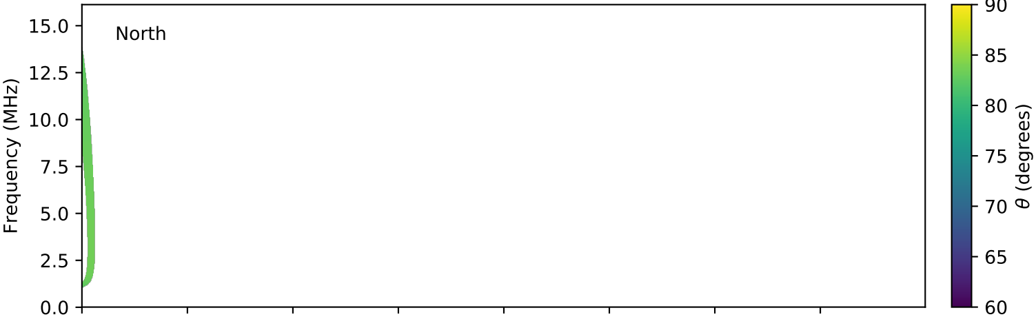
expres_cassini_jupiter_europa_isaac_lossc-wid1deg_3kev_20020119_v01.cdf
