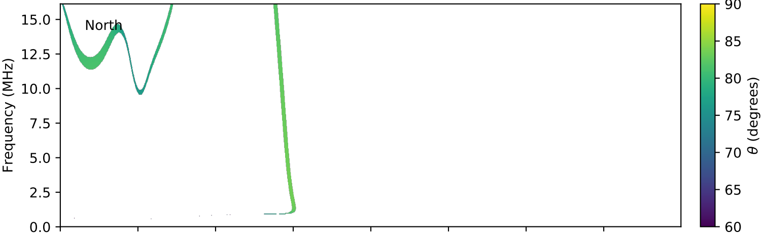
expres_cassini_jupiter_europa_isaac_lossc-wid1deg_3kev_20020115_v01.cdf
