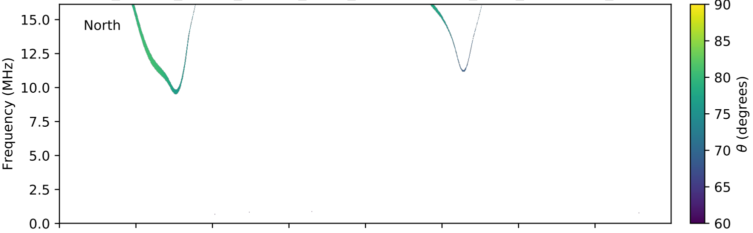
expres_cassini_jupiter_europa_isaac_lossc-wid1deg_3kev_20020114_v01.cdf
