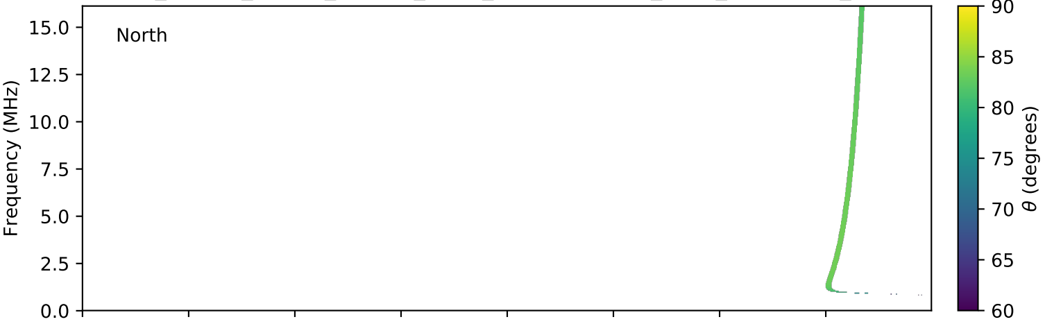
expres_cassini_jupiter_europa_isaac_lossc-wid1deg_3kev_20020113_v01.cdf
