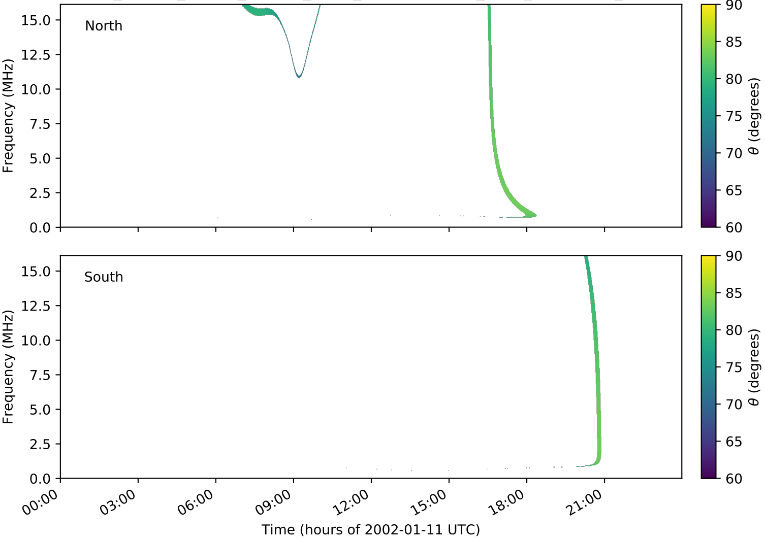
expres_cassini_jupiter_europa_isaac_lossc-wid1deg_3kev_20020111_v01.cdf
