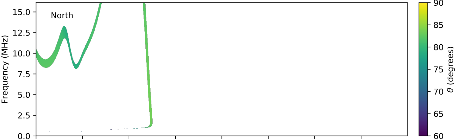
expres_cassini_jupiter_europa_isaac_lossc-wid1deg_3kev_20020108_v01.cdf
