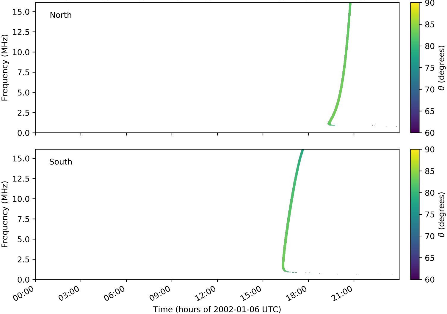
expres_cassini_jupiter_europa_isaac_lossc-wid1deg_3kev_20020106_v01.cdf
