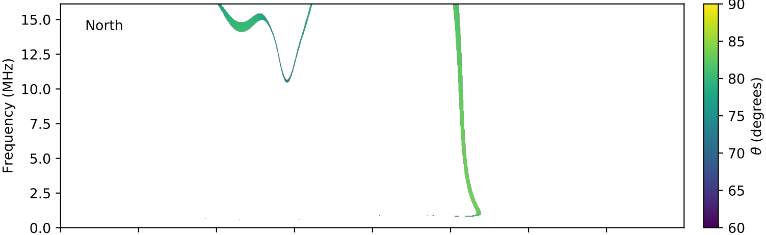
expres_cassini_jupiter_europa_isaac_lossc-wid1deg_3kev_20020104_v01.cdf
