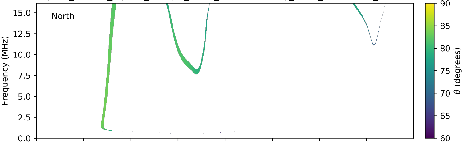
expres_cassini_jupiter_europa_isaac_lossc-wid1deg_3kev_20020103_v01.cdf
