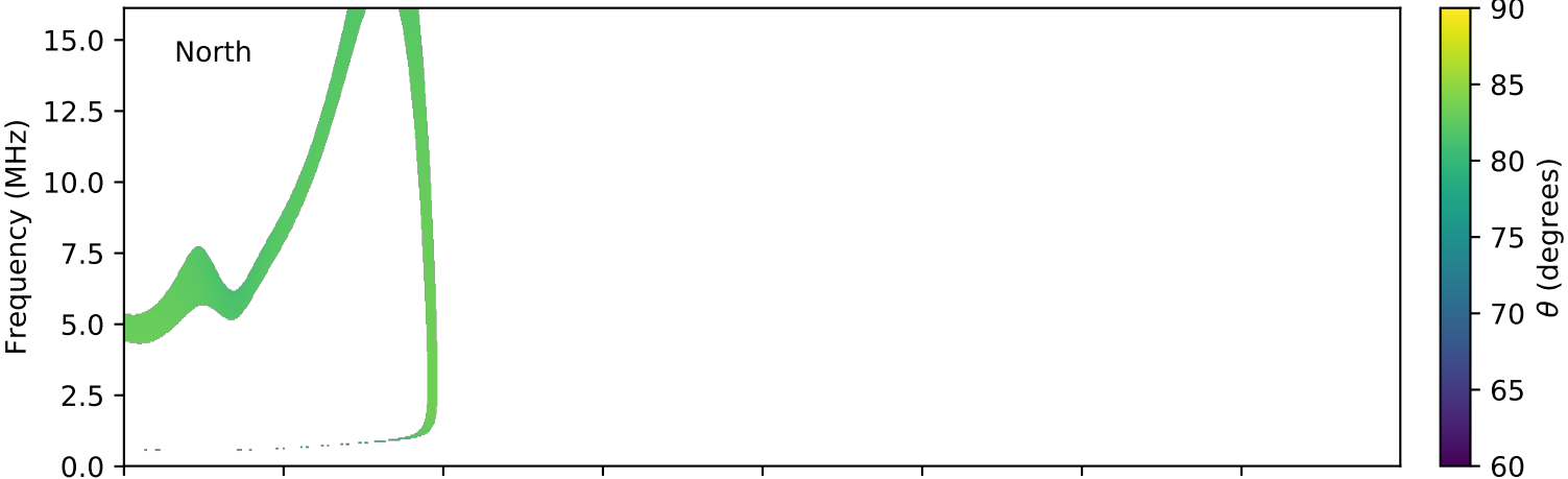
expres_cassini_jupiter_europa_isaac_lossc-wid1deg_3kev_20020101_v01.cdf
