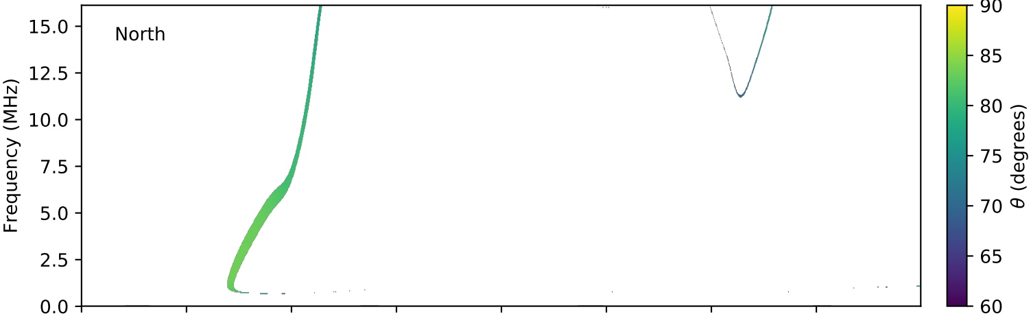
expres_cassini_jupiter_io_isaac_lossc-wid1deg_3kev_20011029_v01.cdf
