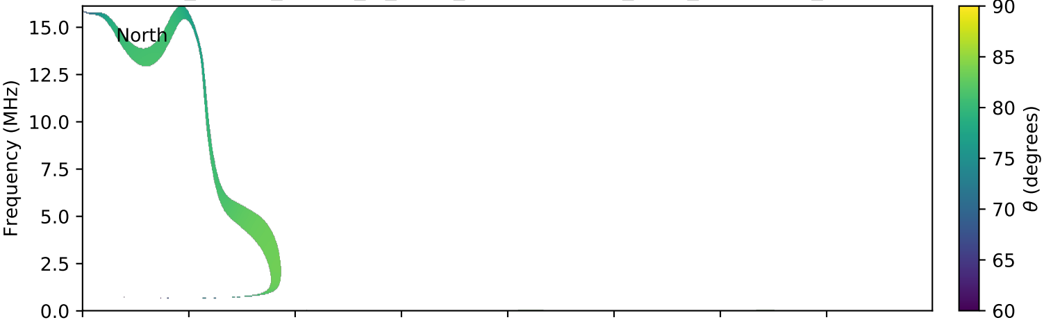
expres_cassini_jupiter_io_isaac_lossc-wid1deg_3kev_20011028_v01.cdf
