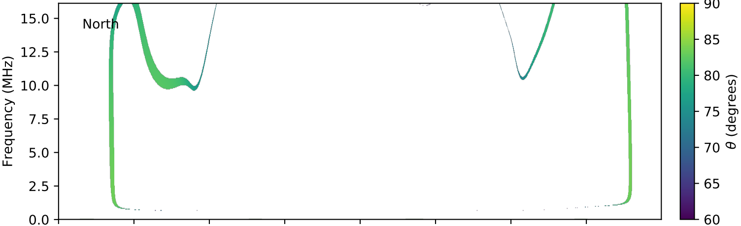
expres_cassini_jupiter_io_isaac_lossc-wid1deg_3kev_20011022_v01.cdf
