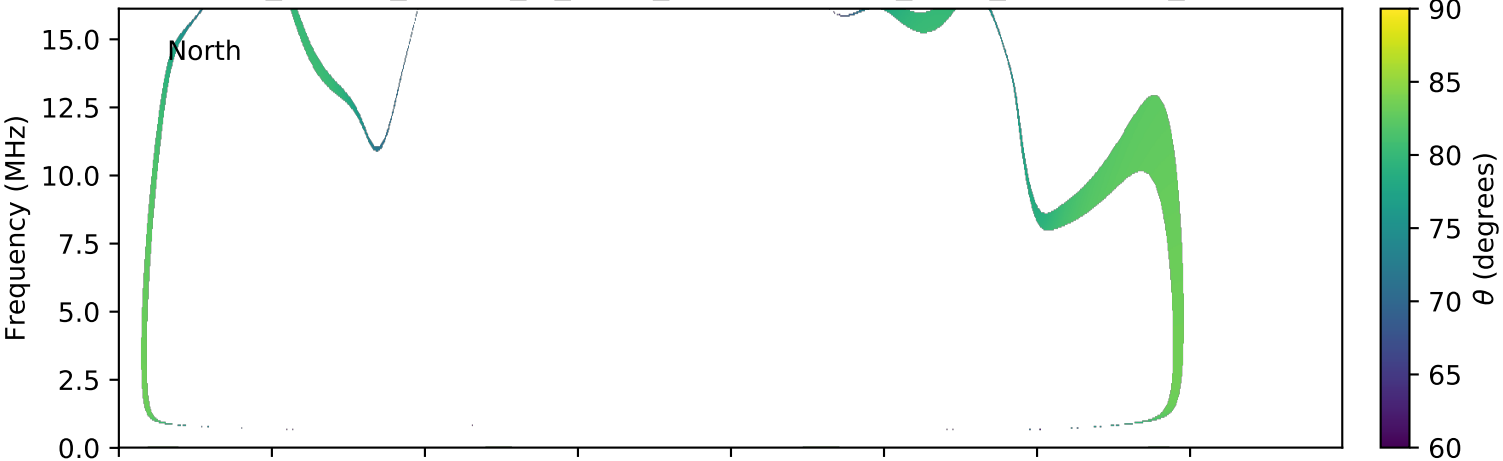
expres_cassini_jupiter_io_isaac_lossc-wid1deg_3kev_20011015_v01.cdf
