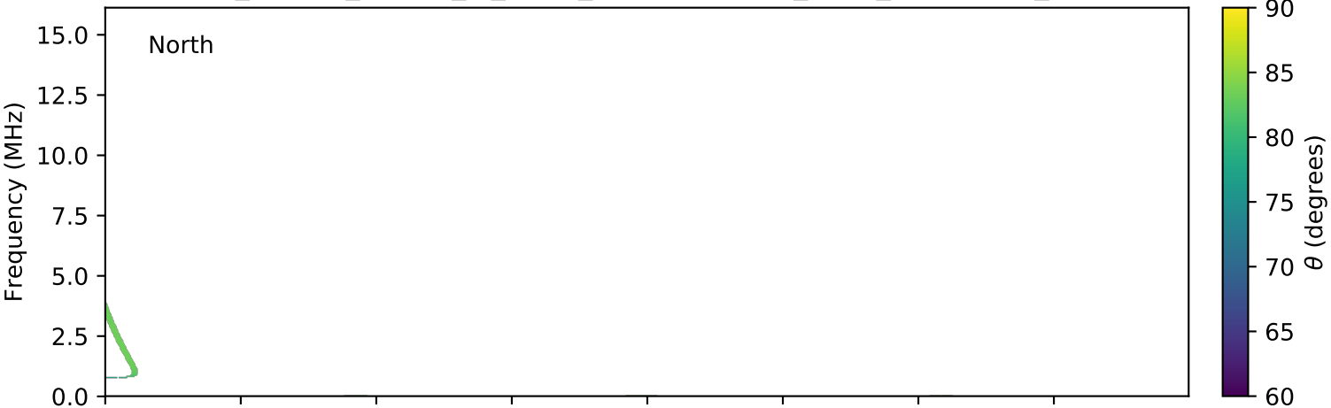
expres_cassini_jupiter_io_isaac_lossc-wid1deg_3kev_20011014_v01.cdf
