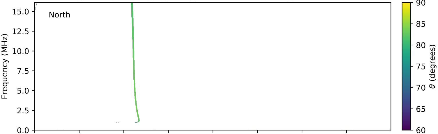
expres_cassini_jupiter_io_isaac_lossc-wid1deg_3kev_20011012_v01.cdf
