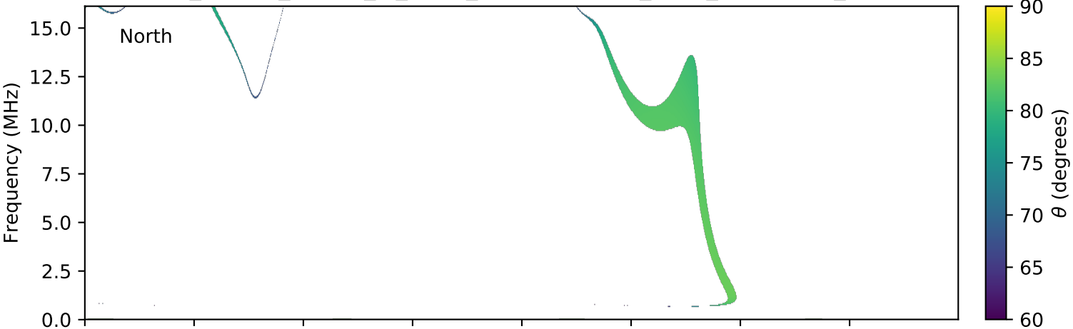
expres_cassini_jupiter_io_isaac_lossc-wid1deg_3kev_20011008_v01.cdf
