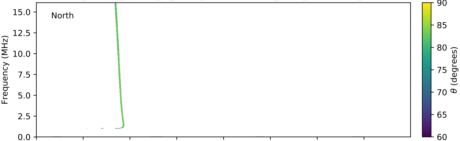
expres_cassini_jupiter_io_isaac_lossc-wid1deg_3kev_20011005_v01.cdf
