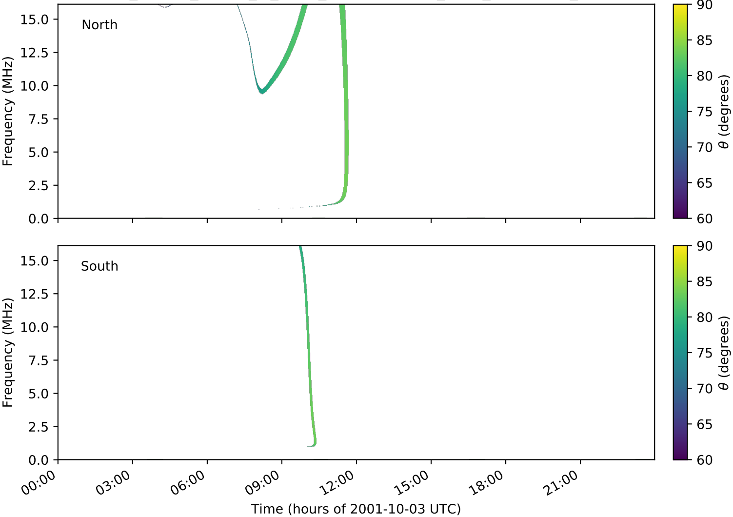
expres_cassini_jupiter_io_isaac_lossc-wid1deg_3kev_20011003_v01.cdf
