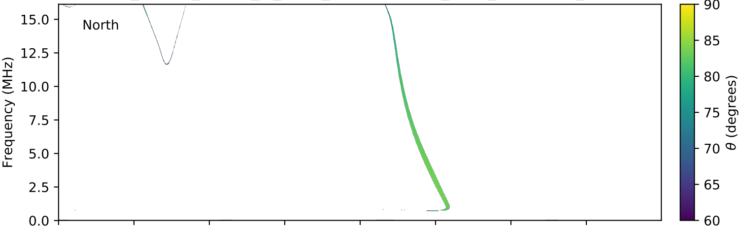
expres_cassini_jupiter_io_isaac_lossc-wid1deg_3kev_20011001_v01.cdf
