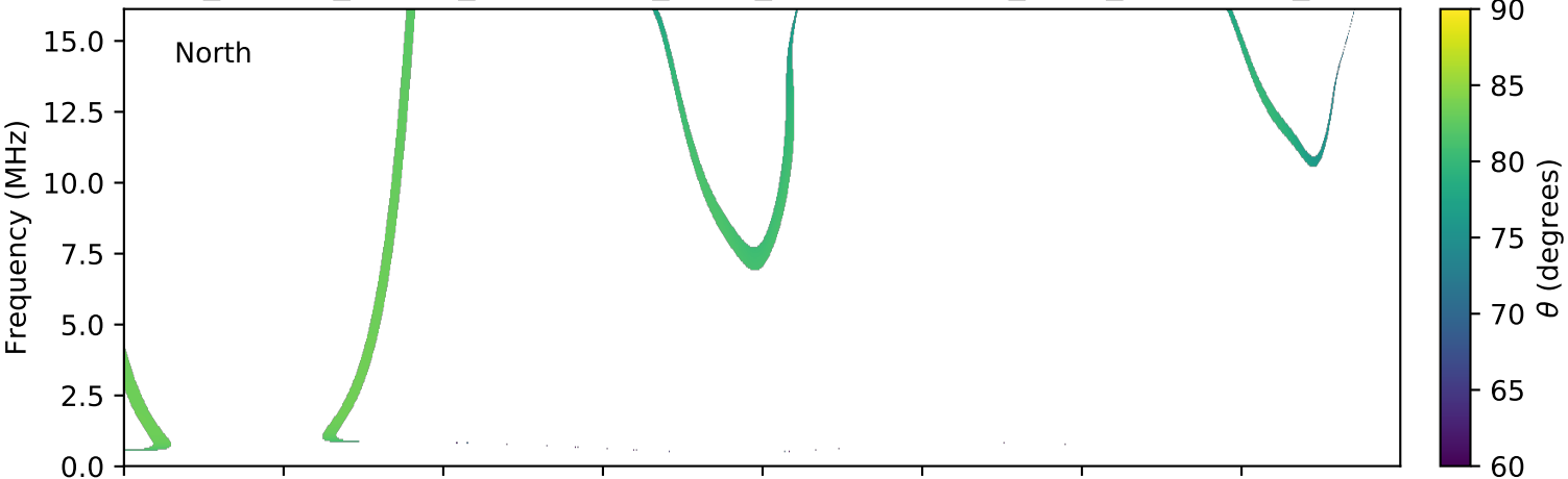
expres_cassini_jupiter_ganymede_isaac_lossc-wid1deg_3kev_20011030_v01.cdf
