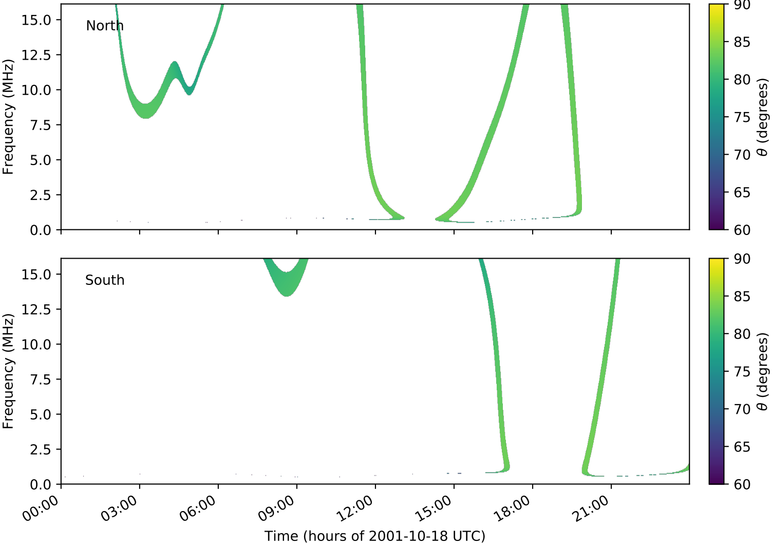
expres_cassini_jupiter_ganymede_isaac_lossc-wid1deg_3kev_20011018_v01.cdf
