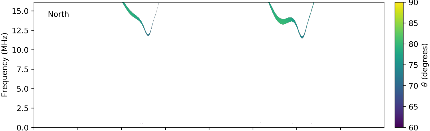
expres_cassini_jupiter_ganymede_isaac_lossc-wid1deg_3kev_20011017_v01.cdf
