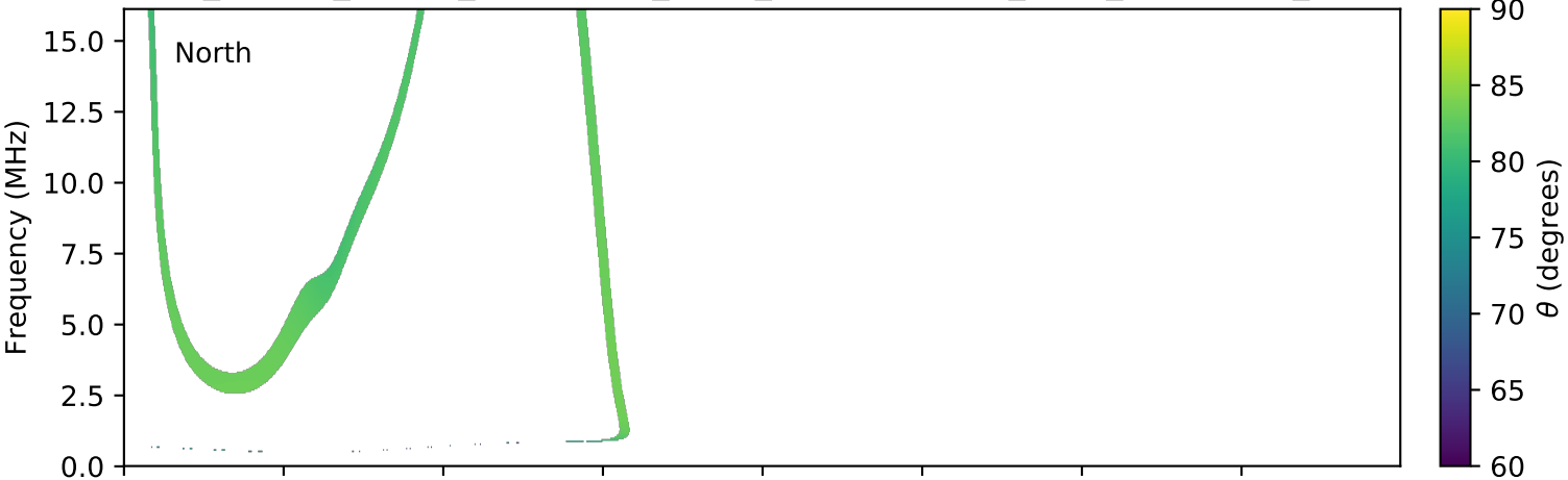
expres_cassini_jupiter_ganymede_isaac_lossc-wid1deg_3kev_20011004_v01.cdf
