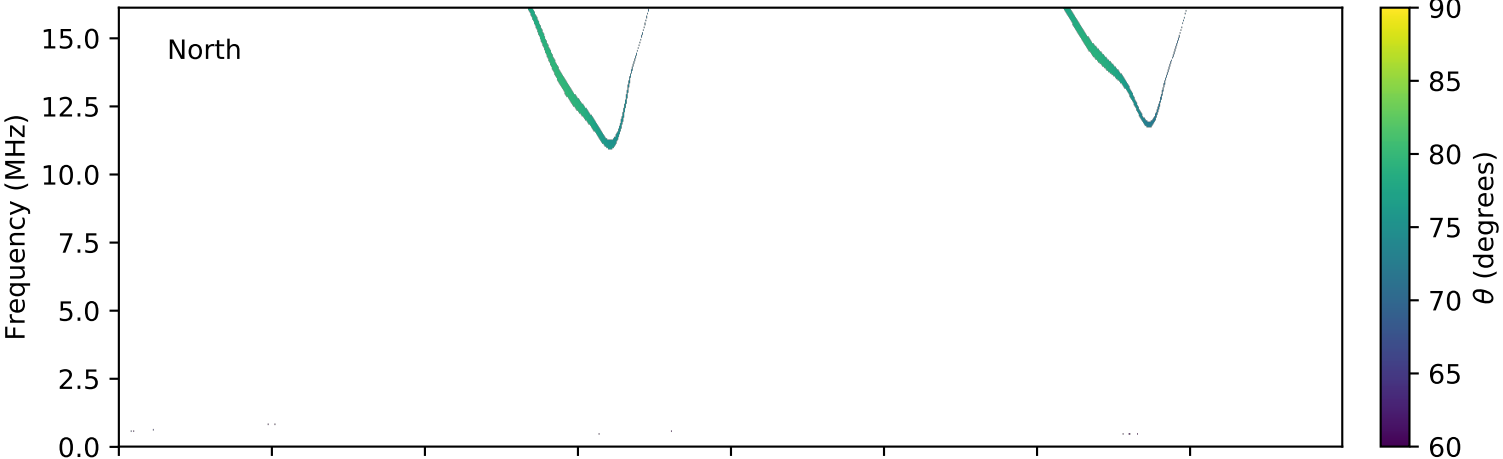
expres_cassini_jupiter_ganymede_isaac_lossc-wid1deg_3kev_20011002_v01.cdf
