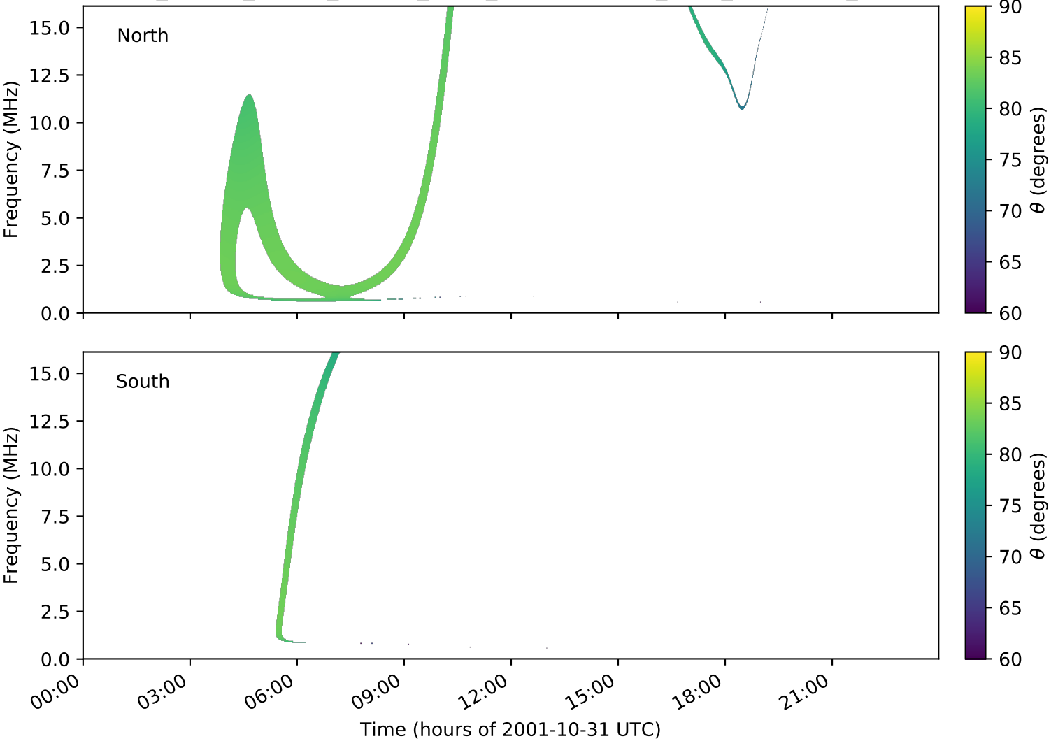
expres_cassini_jupiter_europa_isaac_lossc-wid1deg_3kev_20011031_v01.cdf
